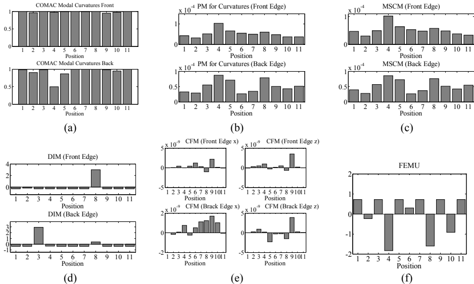
Figure 9 : Damage analysis of model A for the 15 mm crack depth scenario: (a) COMAC values; (b) PM; (c) MSCM; (d) DIM; (e) CFM; and (f) FEMU
