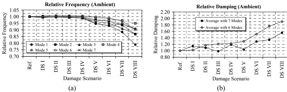
Figure 8 : Dynamic global response: (a) relative frequency variation; and (b) relative damping variation.
