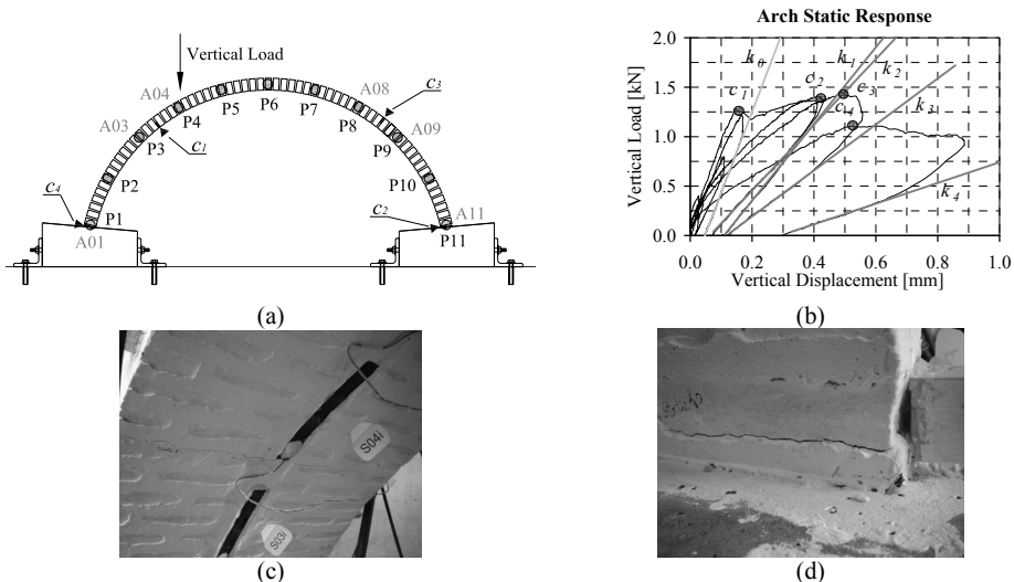
Figure 4 : Static tests: (a) crack locations and sensor positions; (b) static structural response; (c) crack c_1 in the intrados; and (d) crack c_2 at the right support.
