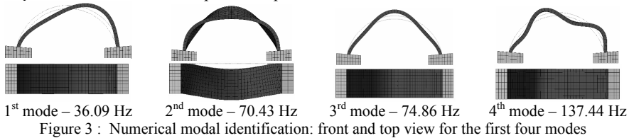
Figure 3 : Numerical modal identification: front and top view for the first four modes
