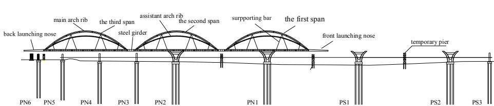
Fig. 2. General layout of launching construction of Jiubao Bridge.
